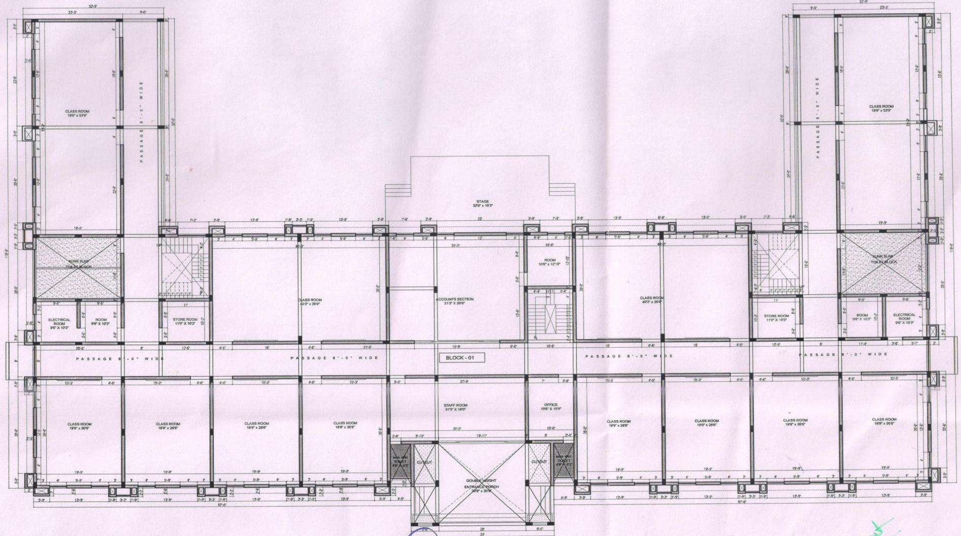
WORKING DRAWING FIRST FLOOR PLAN
